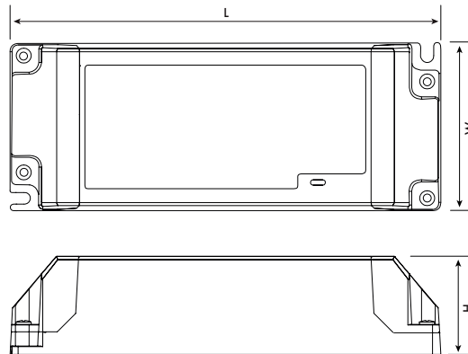
PCV100 & PCV150 Series 100W & 150W Drivers Mechanical
